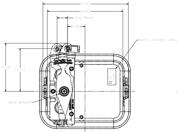
A5020064-001 HANDLE CAR DOOR, INSIDE LEFT HAND SHOWN SCALE: FULL
