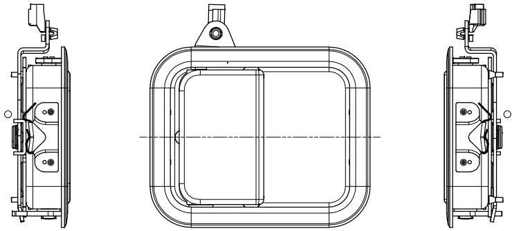
A5020064-001 HANDLE CAR DOOR, INSIDE LEFT HAND SHOWN SCALE: FULL
