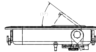
A5020065-001 RH HANDLE SHOWN
