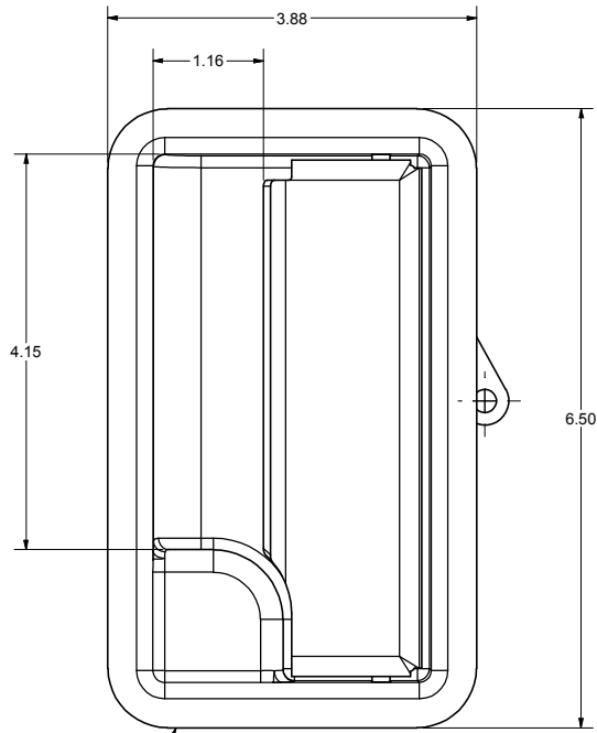
PADDLE HANDLE & RECEPTACLE SUB-ASSEMBLY
