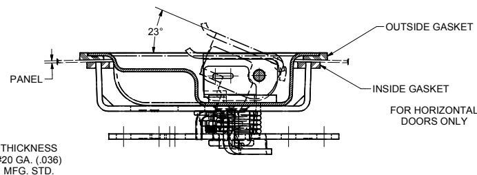
PADDLE HANDLE & RECEPTACLE SUB-ASSEMBLY
