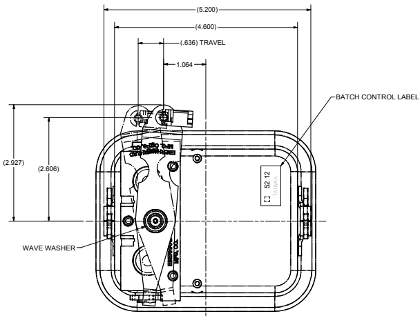
3080799 HANDLE CAB DOOR, INSIDE LEFT HAND SHOWN SCALE: FULL
