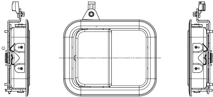
3080799 HANDLE CAB DOOR, INSIDE LEFT HAND SHOWN SCALE: FULL
