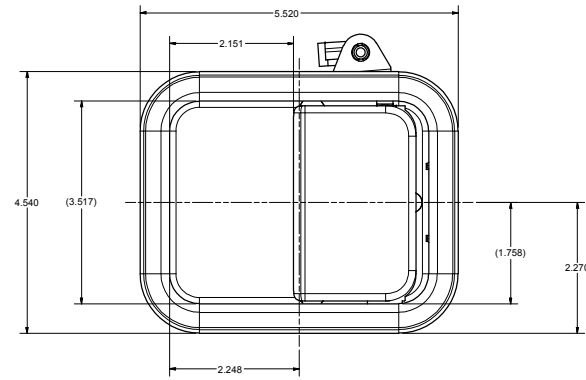
3080800 RH HANDLE SHOWN
