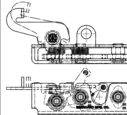
16T-475-L, LEFT HAND LOW PROFILE ROTARY LOCK ASSEMBLY AND THREADED SPACERS
