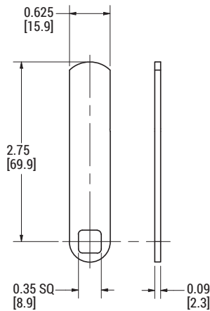
2.75" Straight Cam
