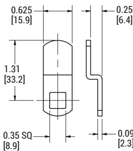
1.313" x .25" Offset Cam
