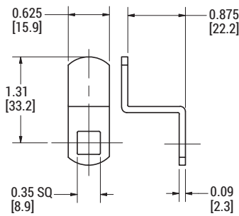
1.313" x .875" Offset Cam
